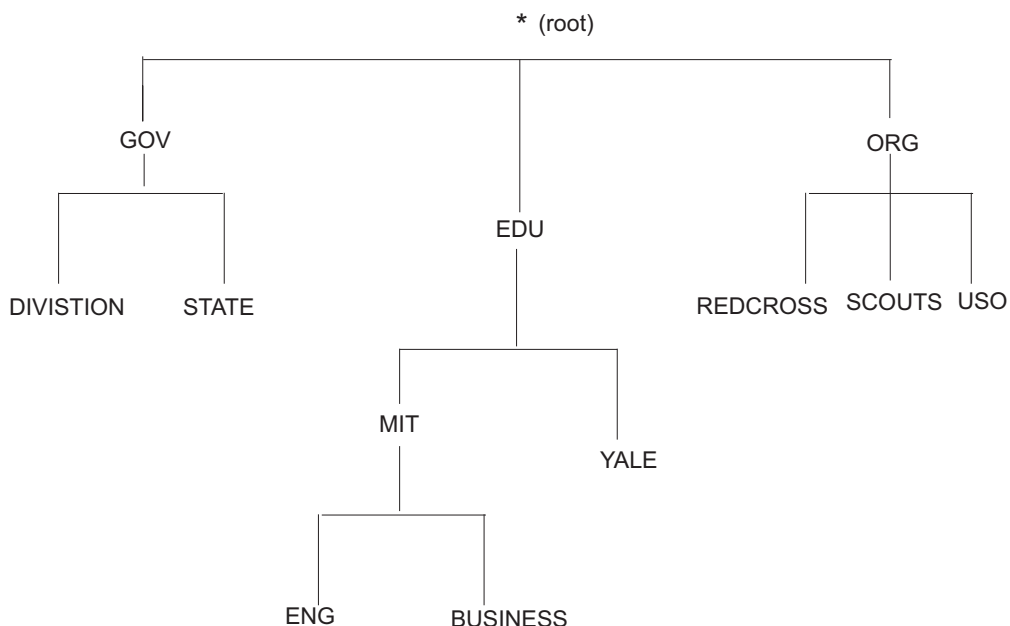
Figure 26. Hierarchical Tree
